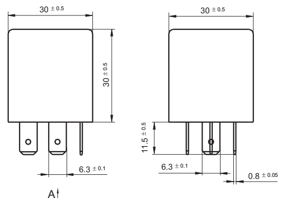
Outline Dimensions
