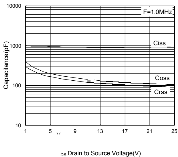
Fig.7 Capacitance
