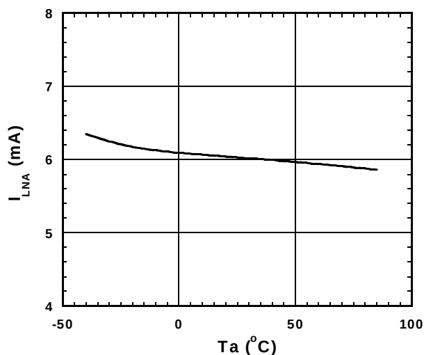
I_{\text{LNA}} vs. Ta
