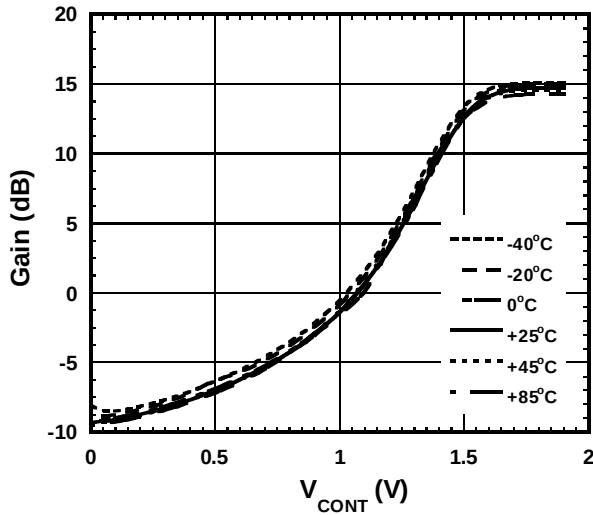
Gain vs. V_{\text{CONT}} (Variable T_a )
