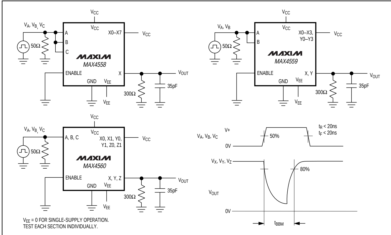
Figure 2. Break-Before-Make Interval
