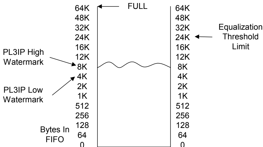
Figure 7 Ingress FIFO Representation
