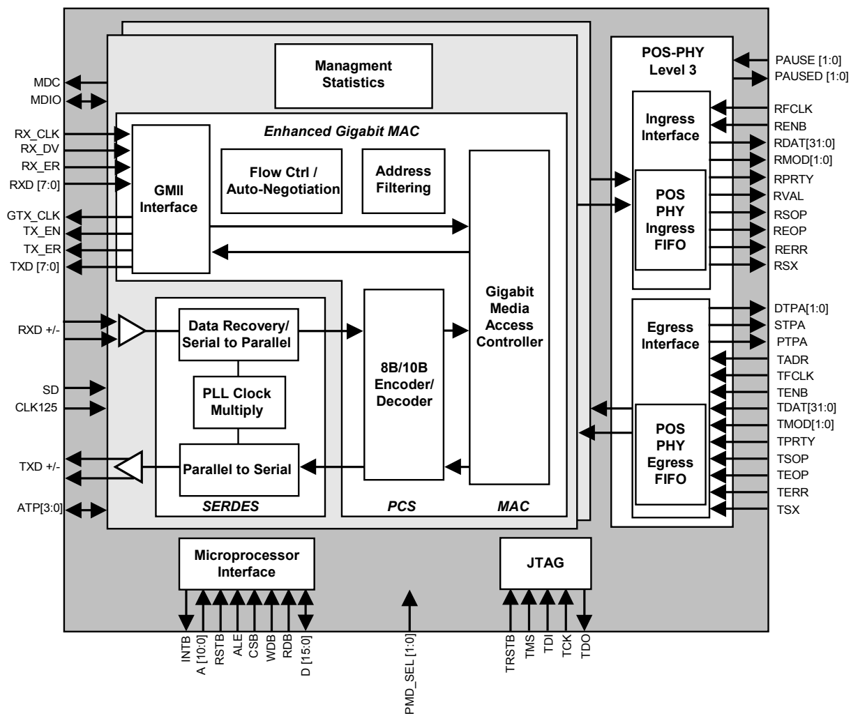
Figure 2 - PM3386 Dual Gigabit Ethernet to POS-PHY Level 3
