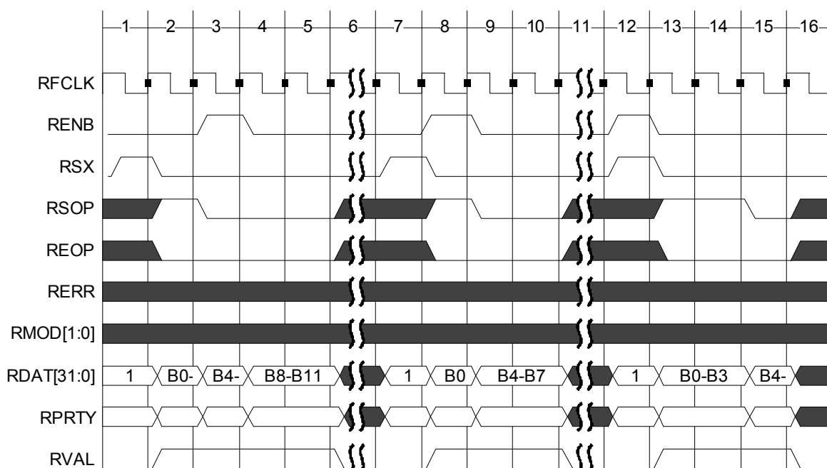
Figure 13 - PM3386 POS-PHY L3 Receive Logical Timing Cases A
