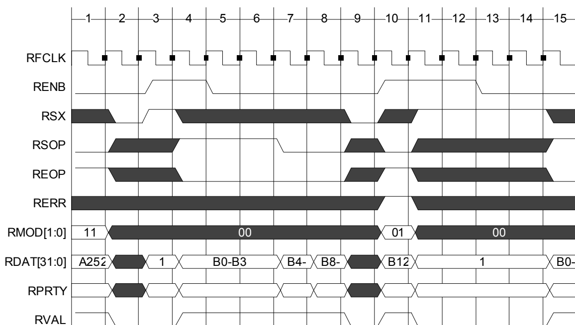
Figure 12 - PM3386 POS-PHY L3 Receive Logical Timing with Pausing
