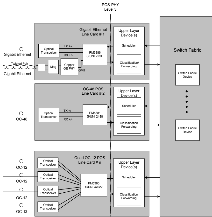
Figure 1 PM3386 Typical Application Example
