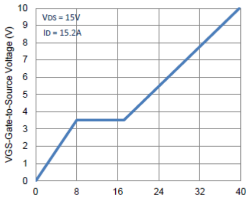
Qg - Total Gate Charge (nC) 7. Gate Charge
