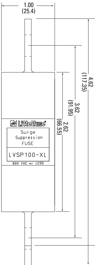
Bolt-In 100 A
