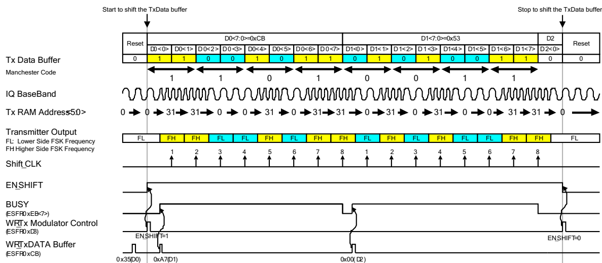
Figure 3-12. Timing Diagram of 1-Byte FSK Data Transmission
