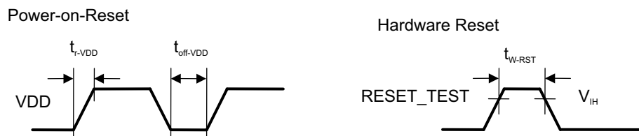
Figure 5-3. Power-on-Reset and Hardware Reset
