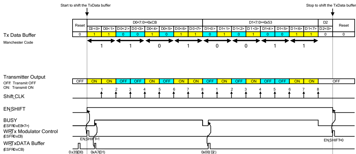
Figure 3-13. Timing Diagram of 1-Byte ASK Data Transmission
