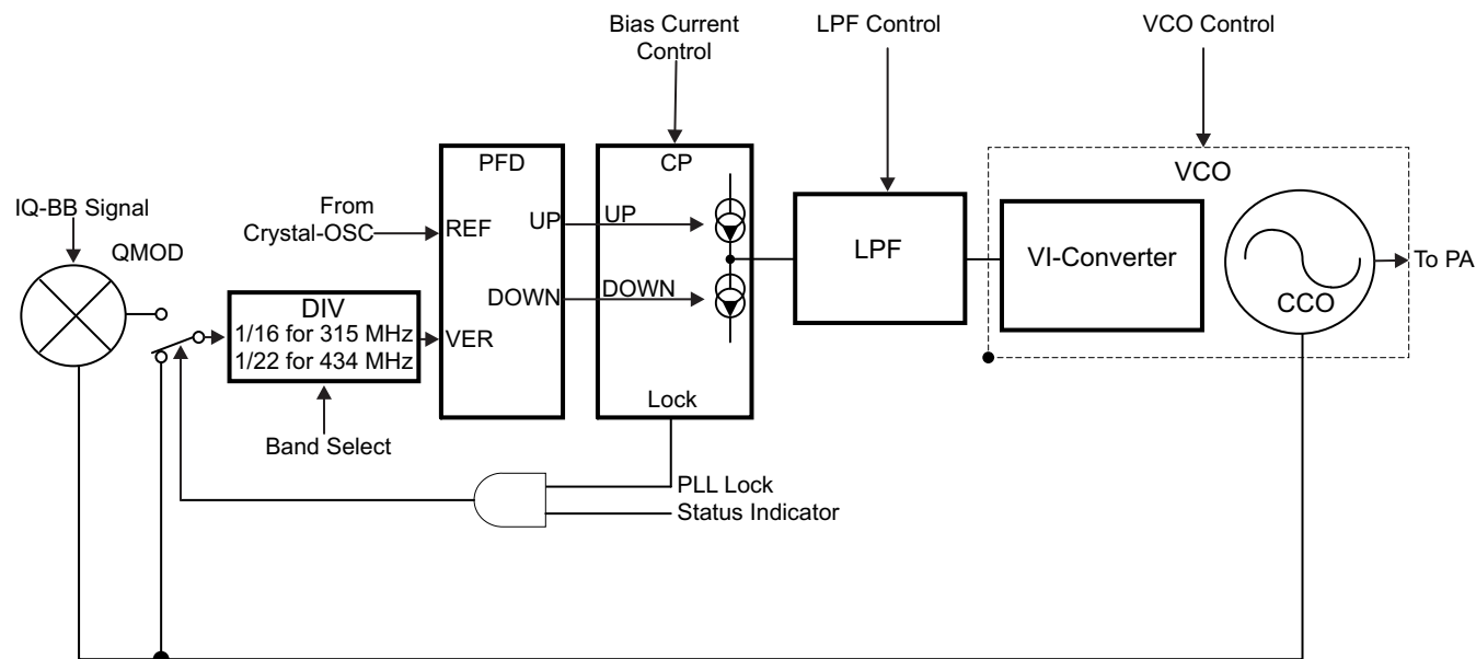
Figure 3-11. PLL Block
