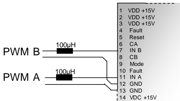
Figure 3.5 Input signals
