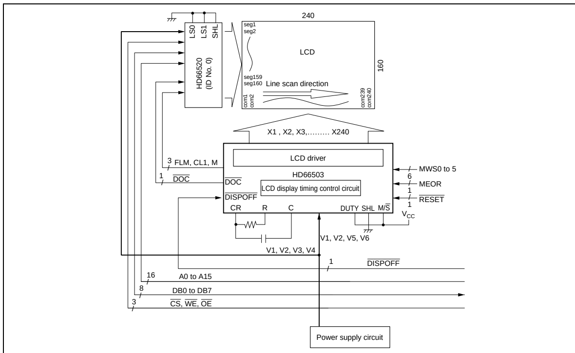
Figure 11 System Configuration (1)
