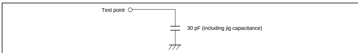
Figure 22 Load Circuit
