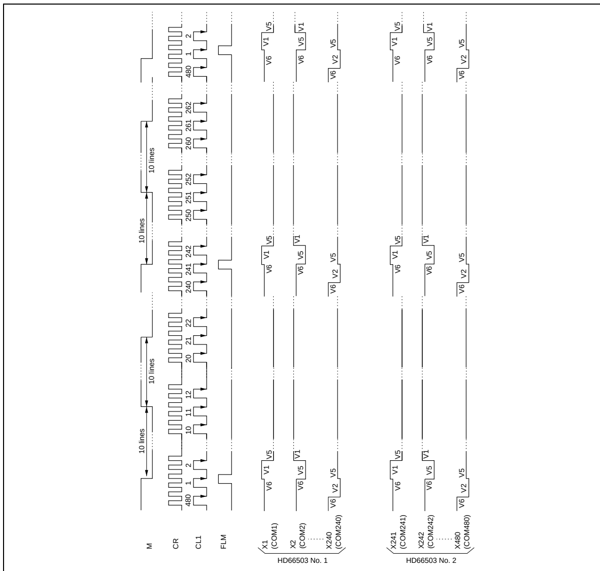
Figure 15 Timing Chart (2)
