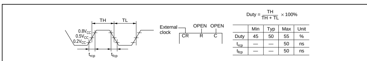
Figure 17 External Clock
