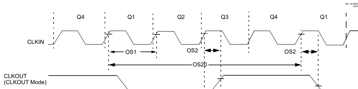
Figure 38-5. Clock Timing
