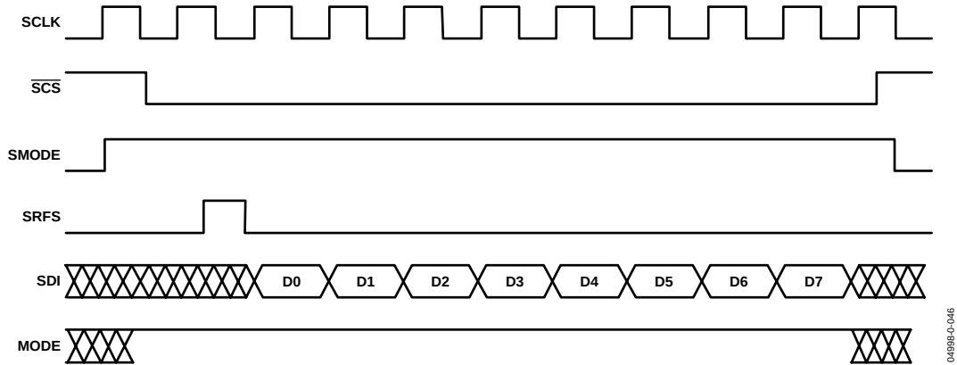
Figure 46. SPORT Serial Write
