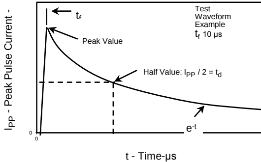
Fig.1 Pulse Wave Form Example
