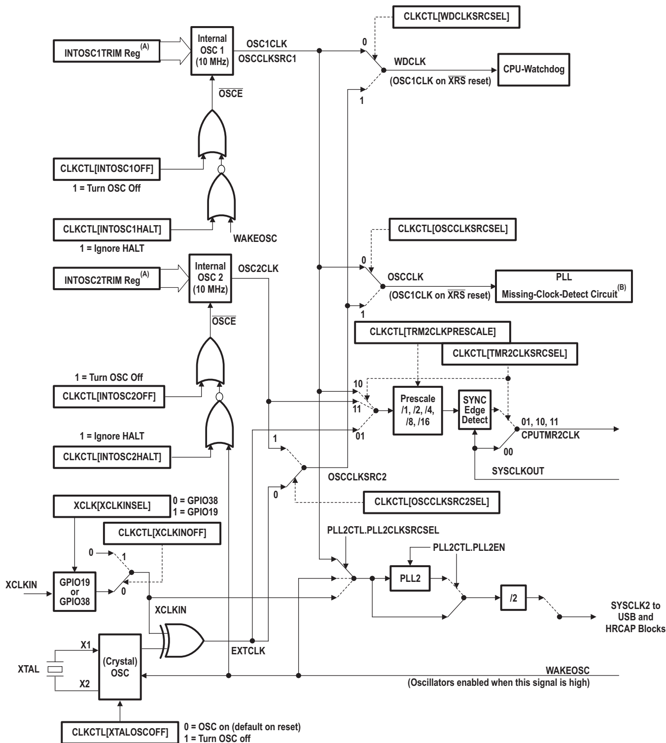
Figure 6-11. Clock Tree
