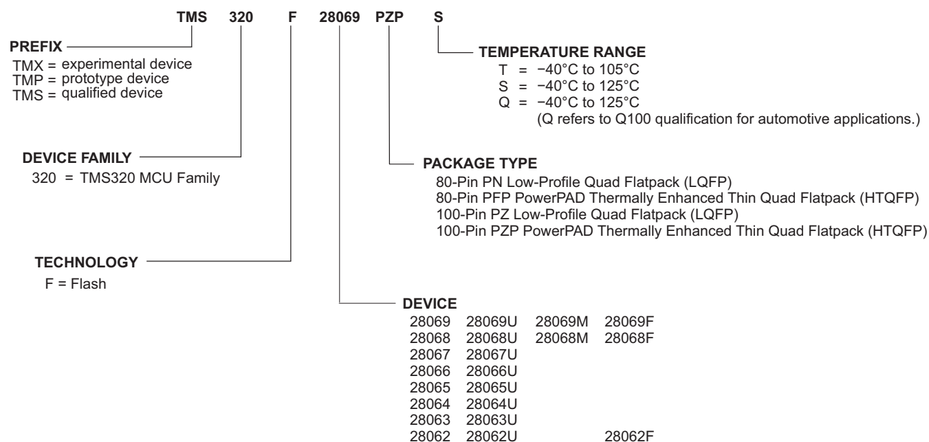
Figure 8-1. Device Nomenclature
