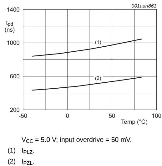
Fig 9. Propagation delay versus temperature
