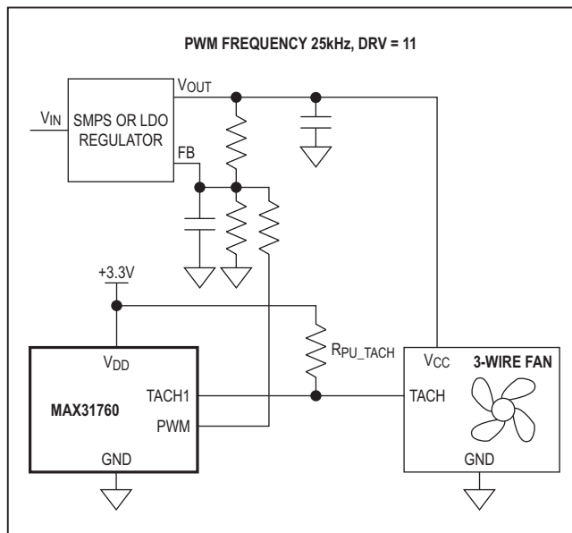
Figure 2c. LDO Regulator Control (3-Wire Fan Driven by Variable Switching Mode Power Supply (SMPS) or LDO Regulator)
