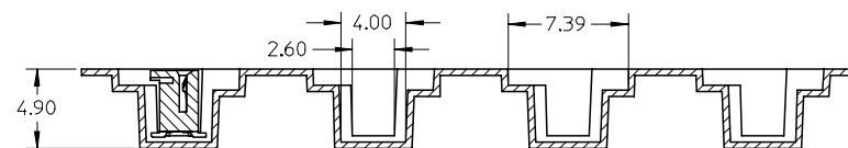
SECTION Z-Z
