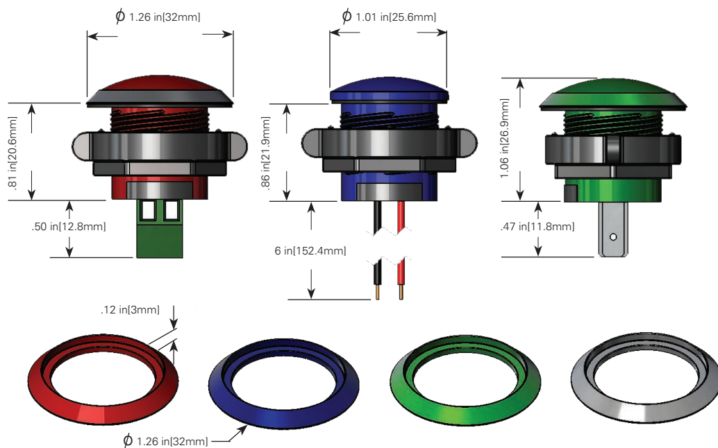
Indicator Assemblies
