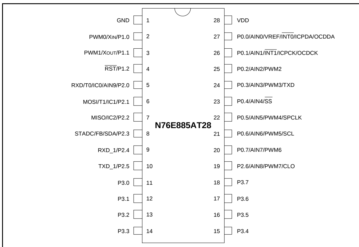
Figure 4-1. Pin Assignment of TSSOP-28 Package
