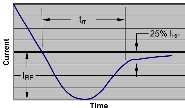
t_{rr} Definition
