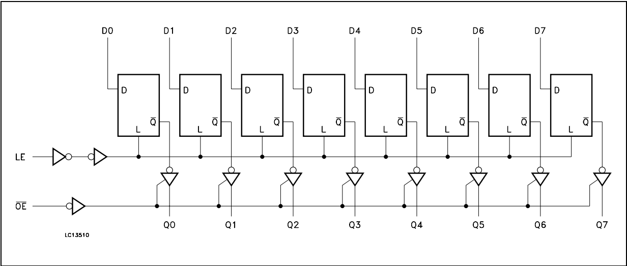
Figure 3: Logic Diagram
