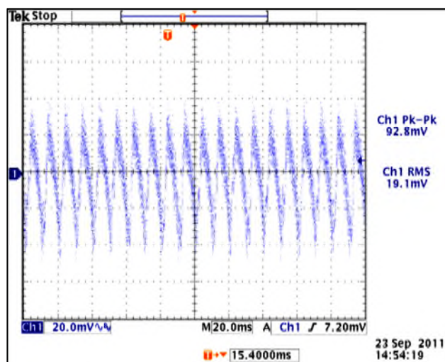
12V OUT, FULL LOAD, 230VAC, 60Hz
