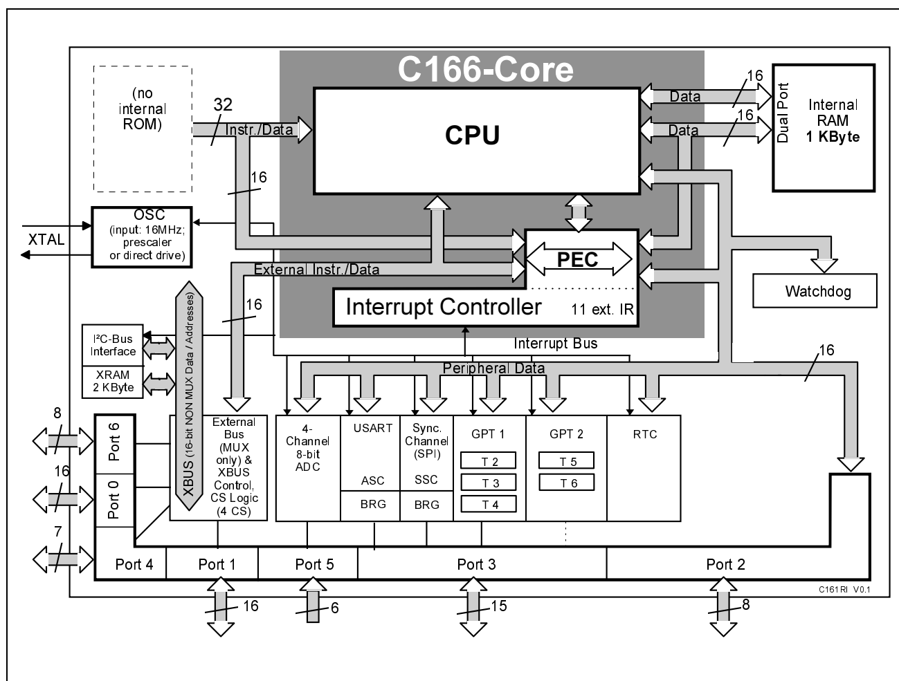
Figure 4 Block Diagram
