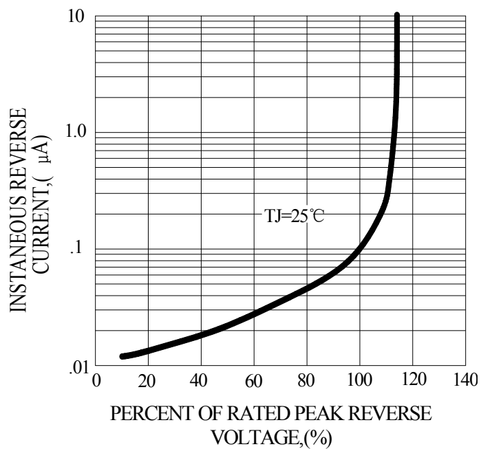
FIG.4-TYPICAL REVERSE CHARACTERISTICS
