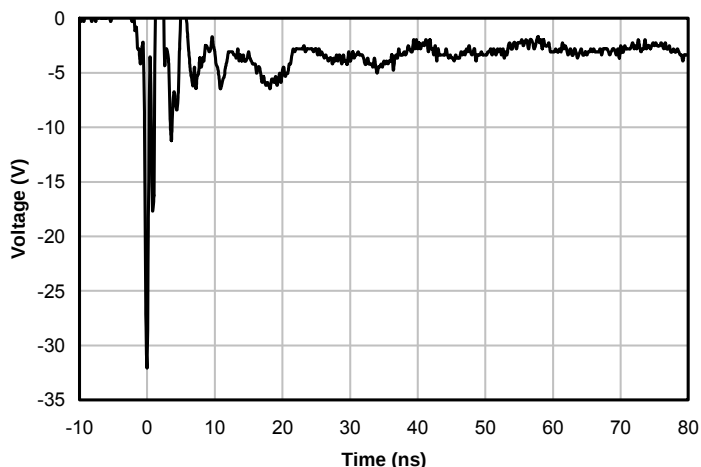
Analog Crosstalk DM, DP, ID Pins (Pins 2, 3, 4)
