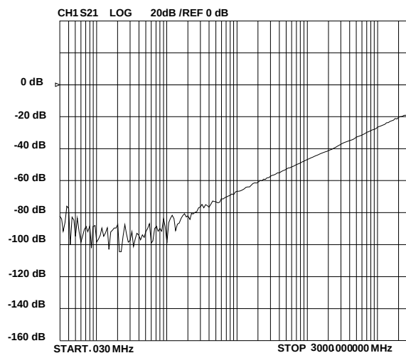
Analog Crosstalk DM, DP, ID Pins (Pins 2, 3, 4)
