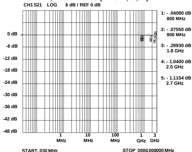
Typical Insertion Loss S21 DM, DP, ID Pins (Pins 2, 3, 4)
