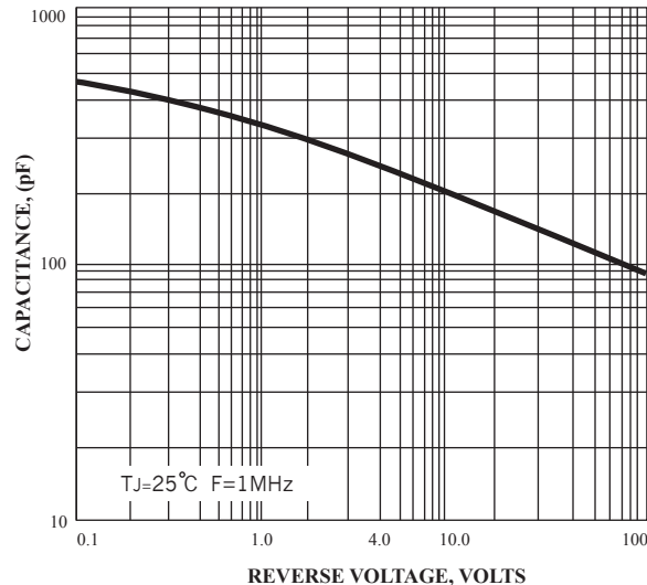
FIG.4-TYPICAL JUNCTION CAPACITANCE
