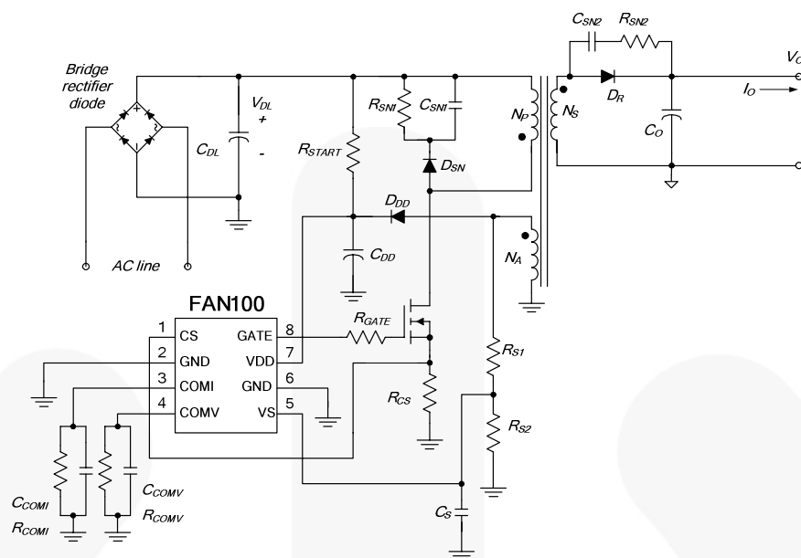
Figure 2. Typical Application
