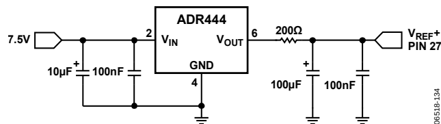
Figure 54. Reference Connection
