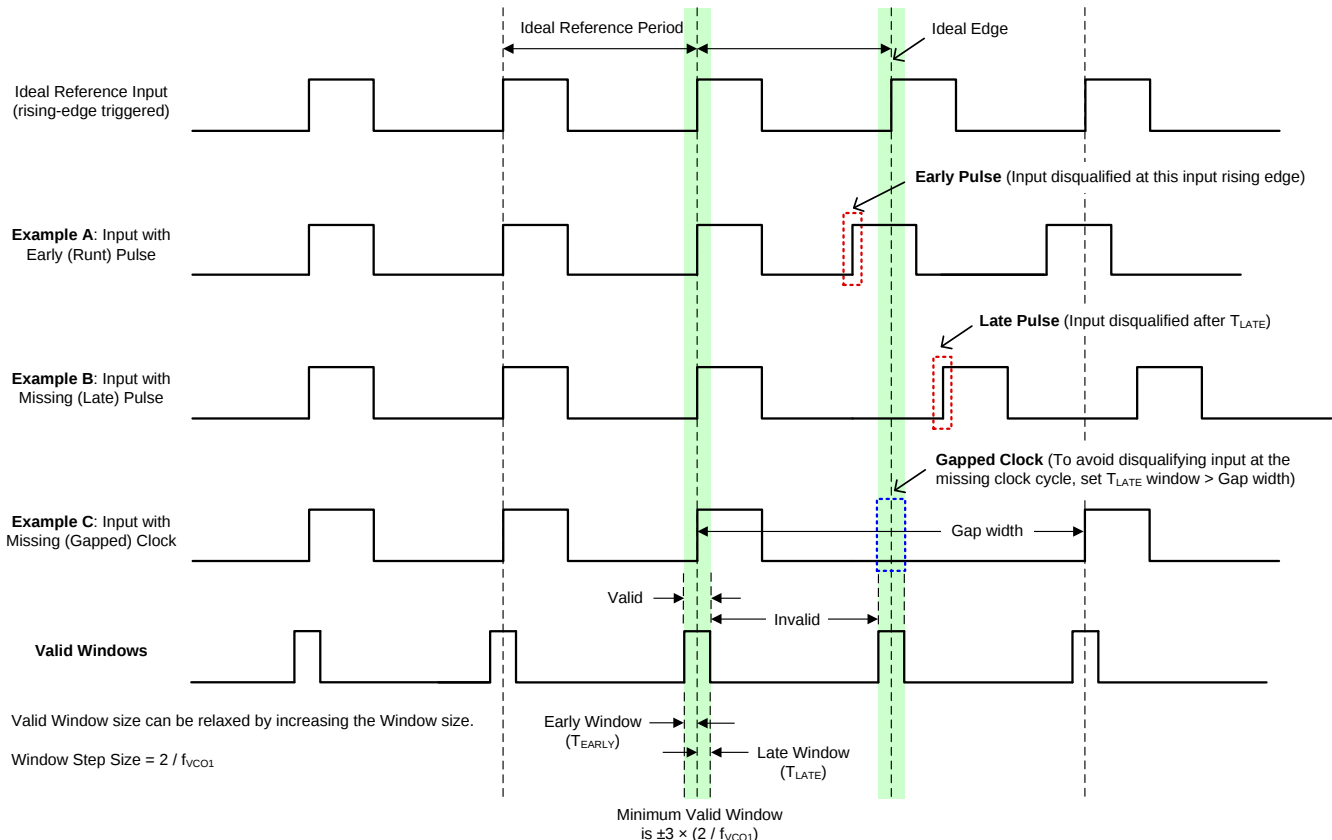
图 38. Early and Late Window Detector Examples
