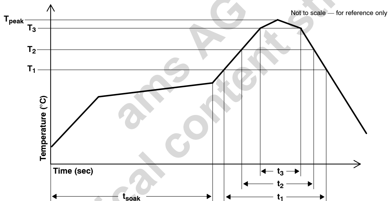
Figure 10. TSL257T Solder Reflow Profile
