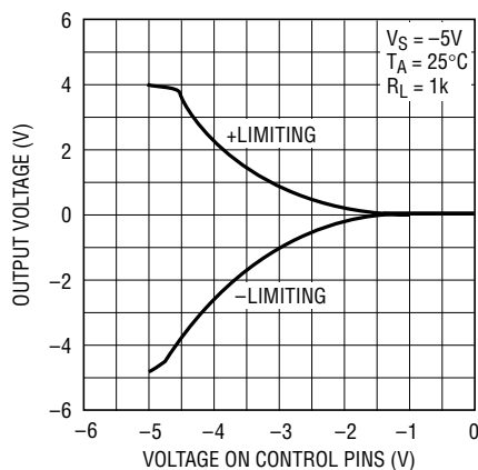
Output Voltage vs Voltage On Control Pins
