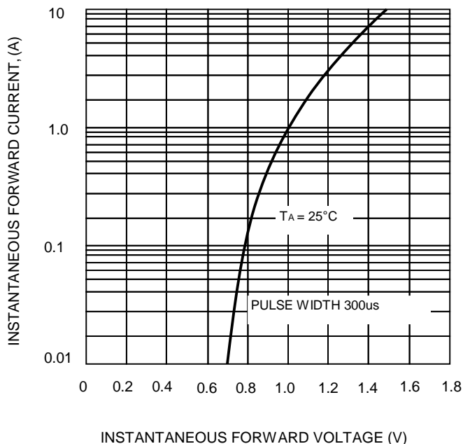
FIG.2-TYPICAL FORWARD CHARACTERISTICS
