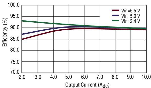
Fig. 3 Efficiency vs. Output Current ( V_{out} = 1.5 V_{dc} )
