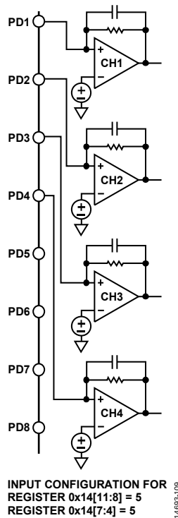
Figure 19. PD1 to PD4 Connection
