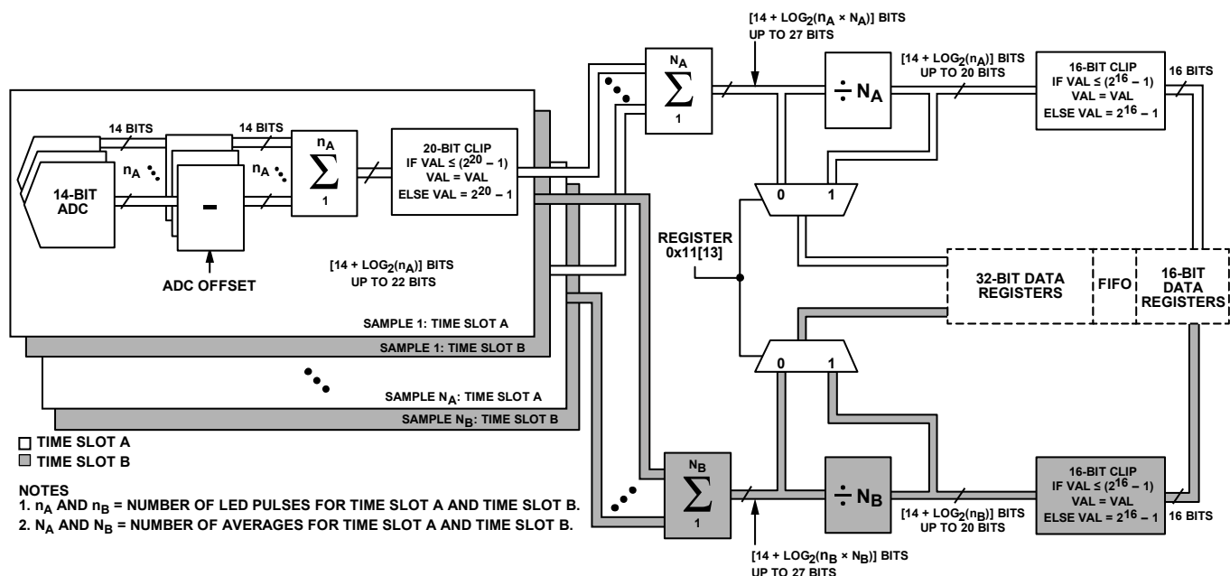
Figure 25. ADPD105/ADPD106/ADPD107 Datapath
