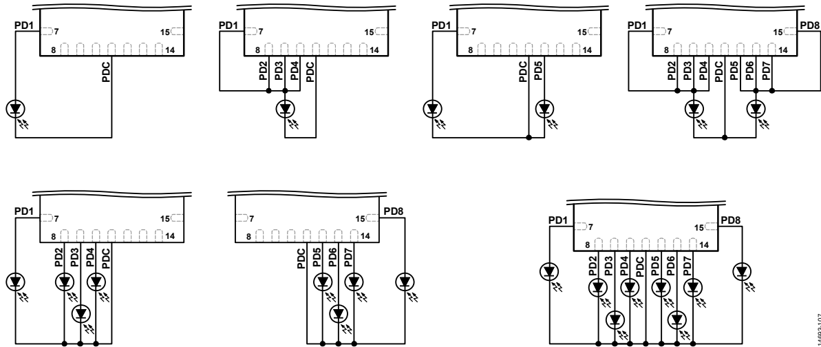
Figure 37. Photodiode Configuration Options for the ADPD105 LFCSP
