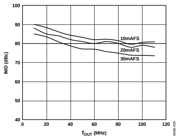
Figure 16. AD9747 IMD vs. Analog Output, 250 MSPS
