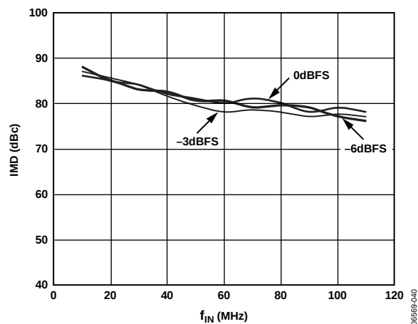
Figure 17. AD9747 IMD vs. Digital Input, 250 MSPS
