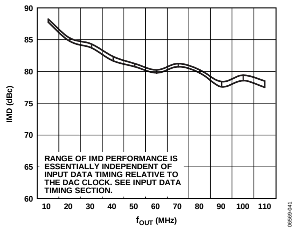
Figure 18. AD9747 IMD vs. f_{OUT} Over Input Data Timing
