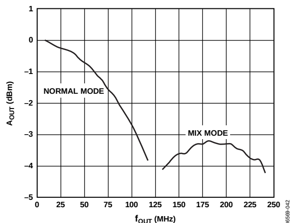
Figure 19. Nominal Power in the Fundamental, I_{FS} = 20 mA
