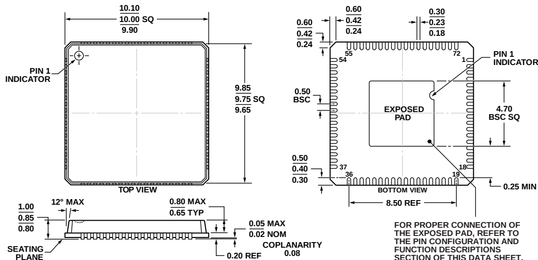
Figure 44. 72-Lead Lead Frame Chip Scale Package [LFCSP_VQ] 10 mm x 10 mm, Very Thin Quad (CP-72-1) Dimensions shown in millimeters
