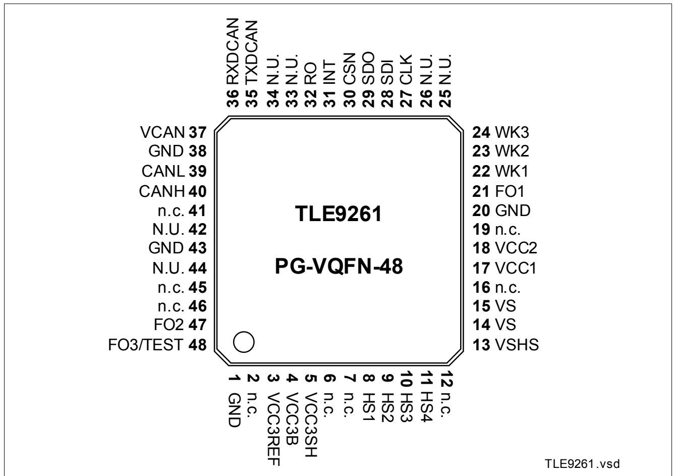
Figure 2 Pin Configuration
