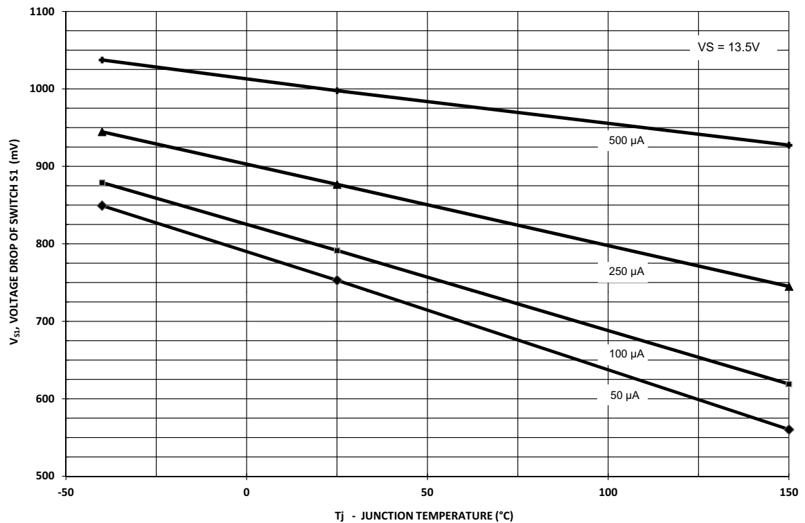
Figure 40 Typical Drop Voltage Characteristics of S1 (between WK1 & WK2)
