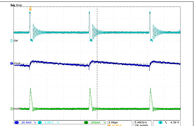
Figure 22. Typical Operation in Power Save Mode ( I_{OUT}=10mA )
