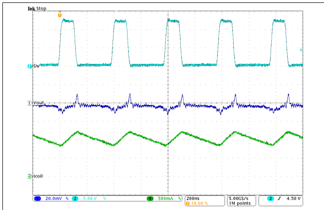
Figure 21. Typical Operation in PWM Mode ( I_{OUT}=1A )
