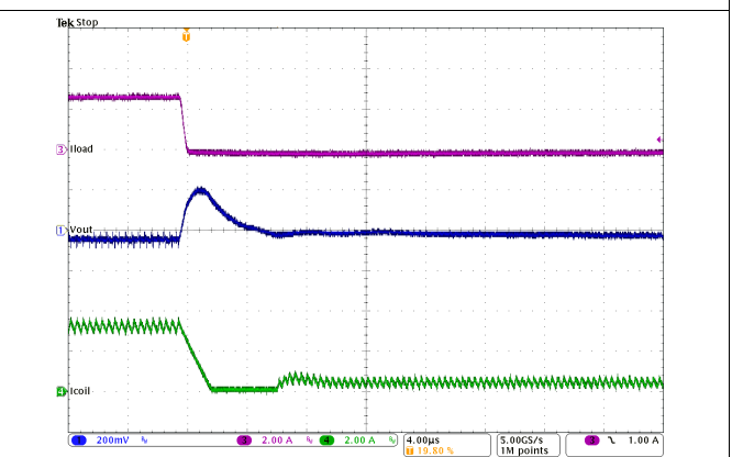
Figure 26. Load Transient Response of Figure 24, Falling Edge
