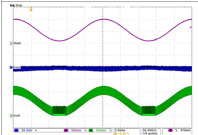
Figure 23. PWM-PSM-Transition
