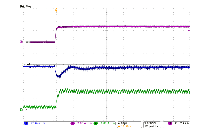
Figure 25. Load Transient Response of Figure 24, Rising Edge
