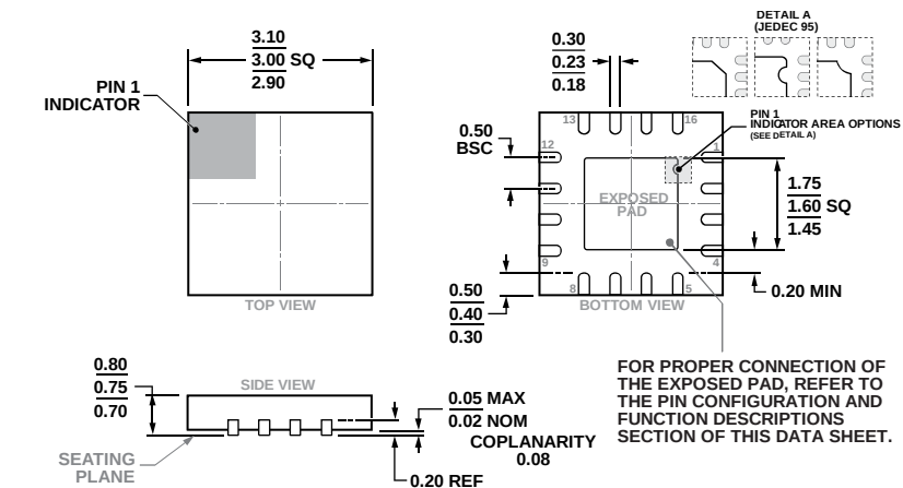
Figure 50. 16-Lead Lead Frame Chip Scale Package [LFCSP] 3 mm x 3 mm Body and 0.75 mm Package Height (CP-16-22) Dimensions shown in millimeters
