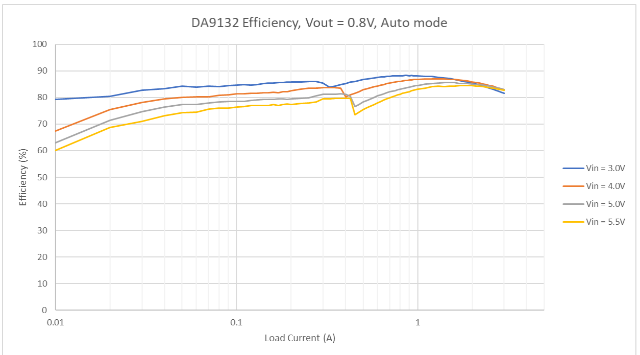
Figure 7: DA9132 Efficiency, V_{OUT} = 0.8 V , Auto Mode
