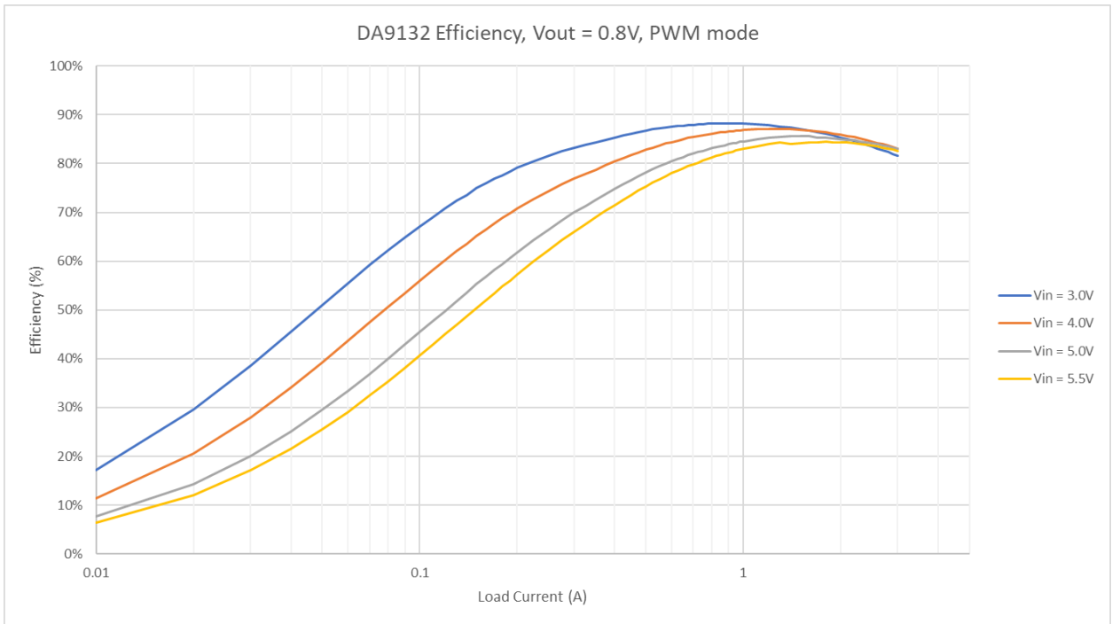
Figure 6: DA9132 Efficiency, V_{OUT} = 0.8 V , PWM Mode
