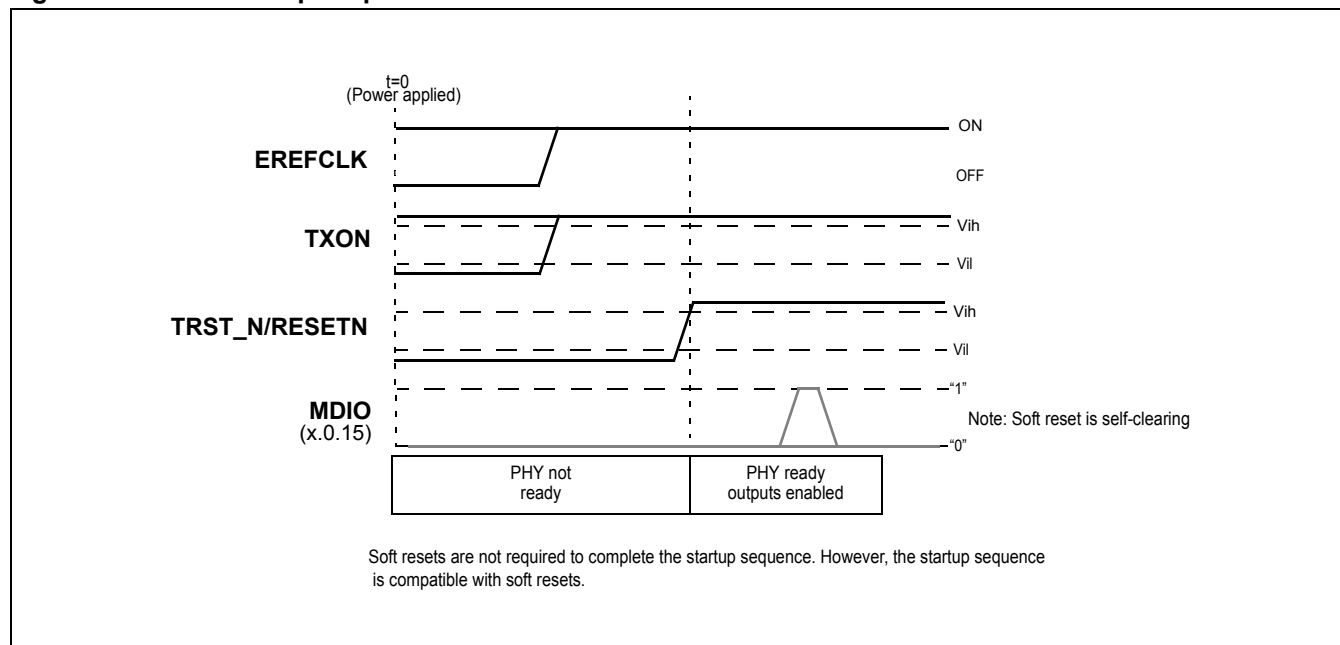
Figure 60: Valid Startup Sequences
