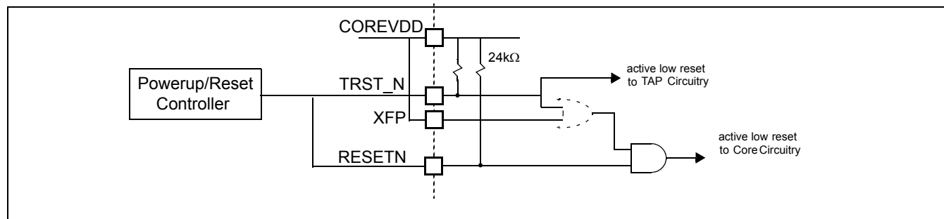
Figure 59: Powerup Reset in a System Application
