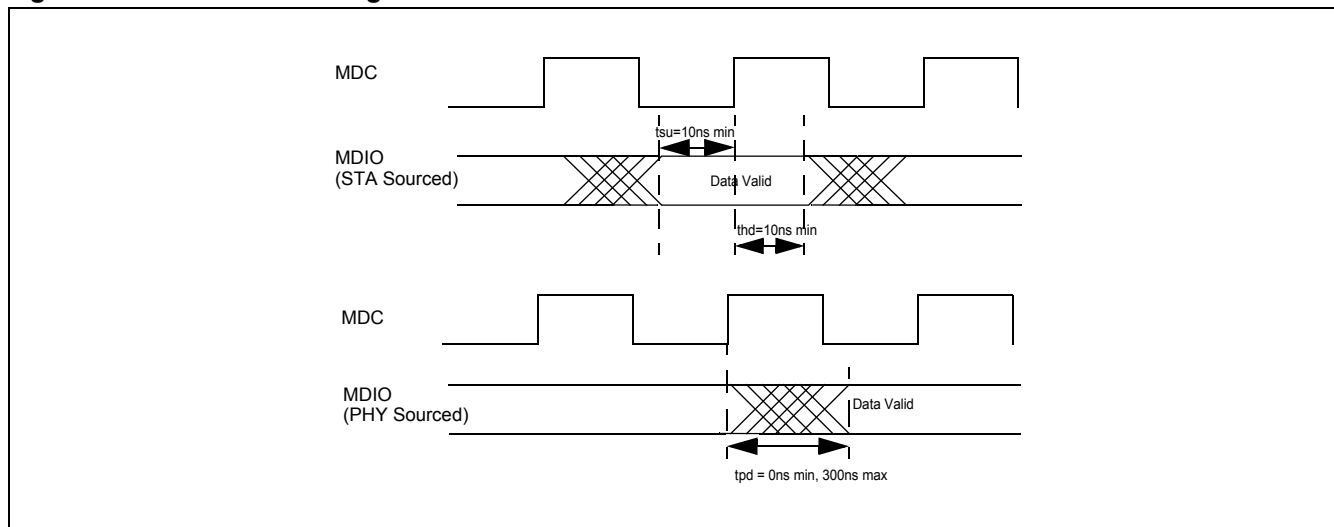
Figure 21: MDIO/MDC Timing
