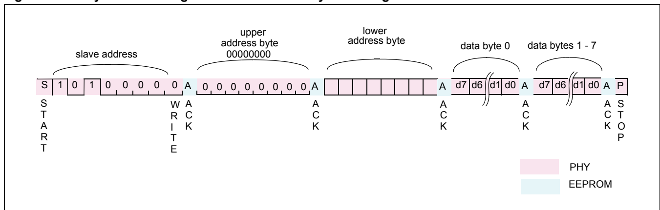
Figure 32: 2-Byte Addressing for EEPROM Write Cycle Timing
