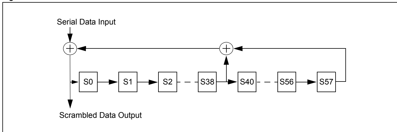
Figure 3: Transmit Scrambler
