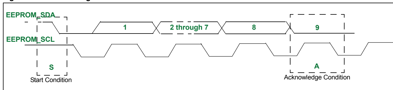
Figure 27: Acknowledge Condition
