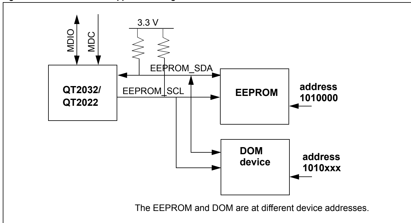
Figure 30: QT2022/32 DOM Application Diagram
