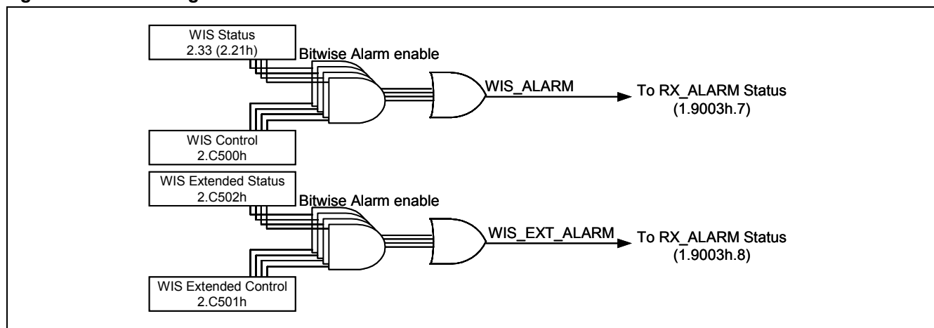
Figure 18: Block diagram of WIS Alarms
