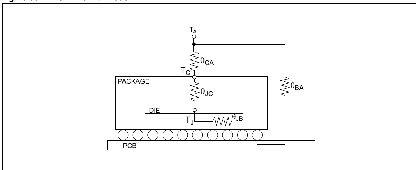
Figure 56: LBGGA Thermal Model
