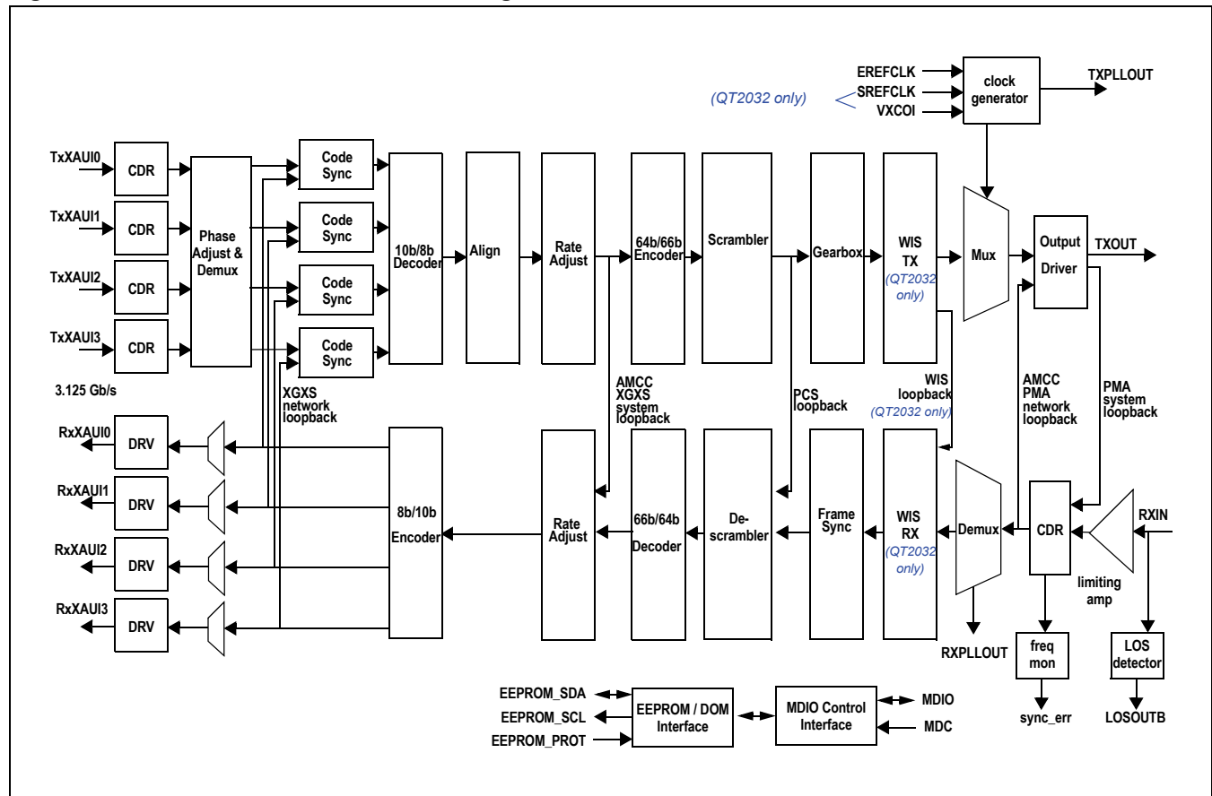
Figure 2: QT2022/32 Functional Block Diagram
