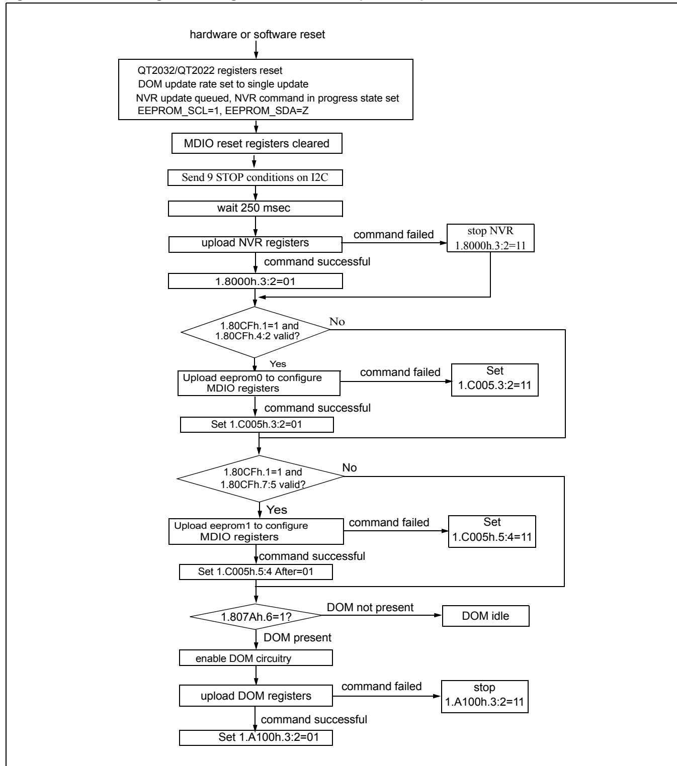
Figure 36: EEPROM Register Configuration and DOM Upload Sequence After Reset
