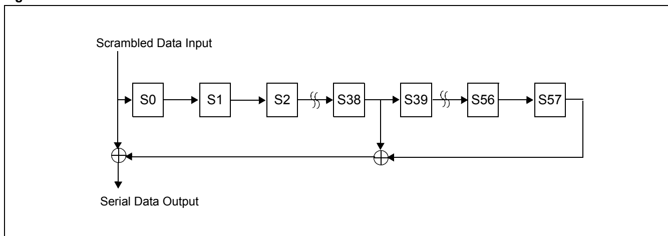
Figure 4: Receive Descrambler
