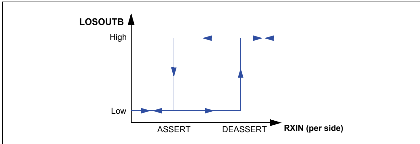
Figure 50: LOSOUTB Hysteresis
