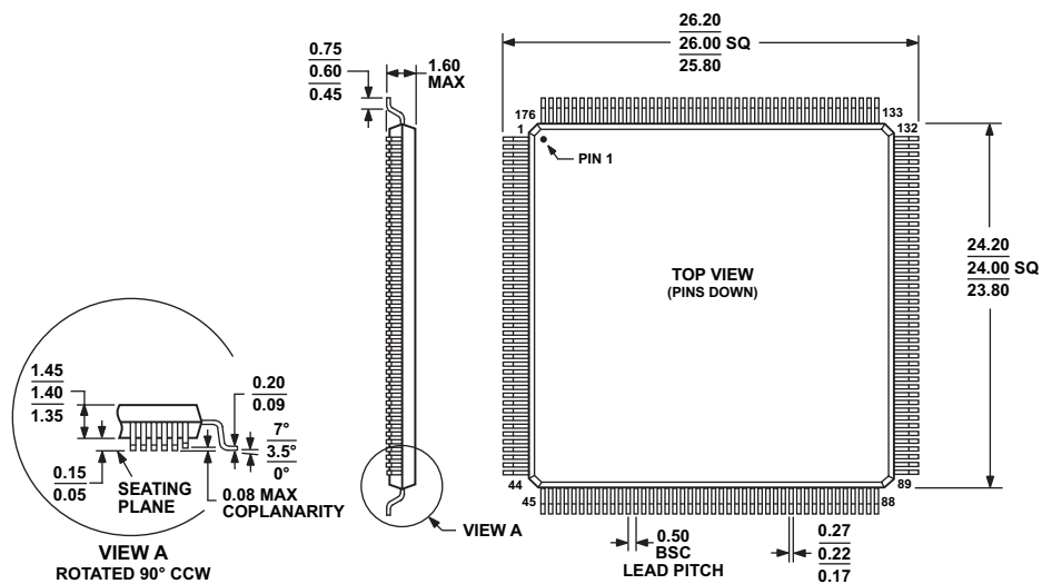
176-LEAD LOW PROFILE QUAD FLAT PACKAGE [LQFP] ST-176
