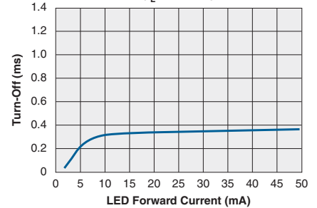
Typical Turn-Off vs. LED Forward Current ( I_L = 120\text{mA} )
