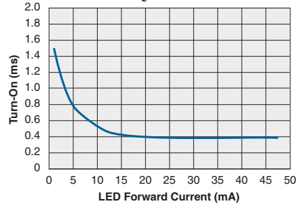
Typical Turn-On vs. LED Forward Current ( I_L = 120\text{mA} )
