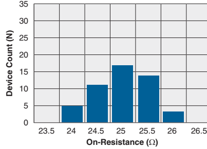
Typical On-Resistance Distribution ( T_A=25^\circ\text{C} , I_L=120\text{mA} , I_F=2\text{mA} )
