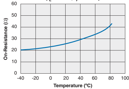
Typical On-Resistance vs. Temperature ( I_L = 80\text{mA} , I_F = 10\text{mA} )
