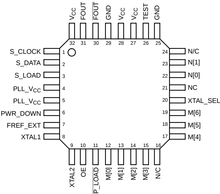
Figure 3. 32-Lead LQFP (Top View)
