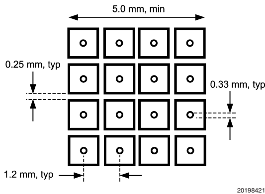
FIGURE 16. Recommended Package Land Pattern
