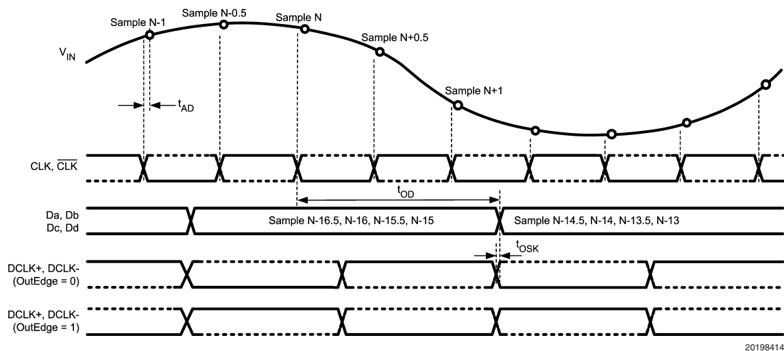
FIGURE 3. ADC082500 Timing — SDR Clocking
