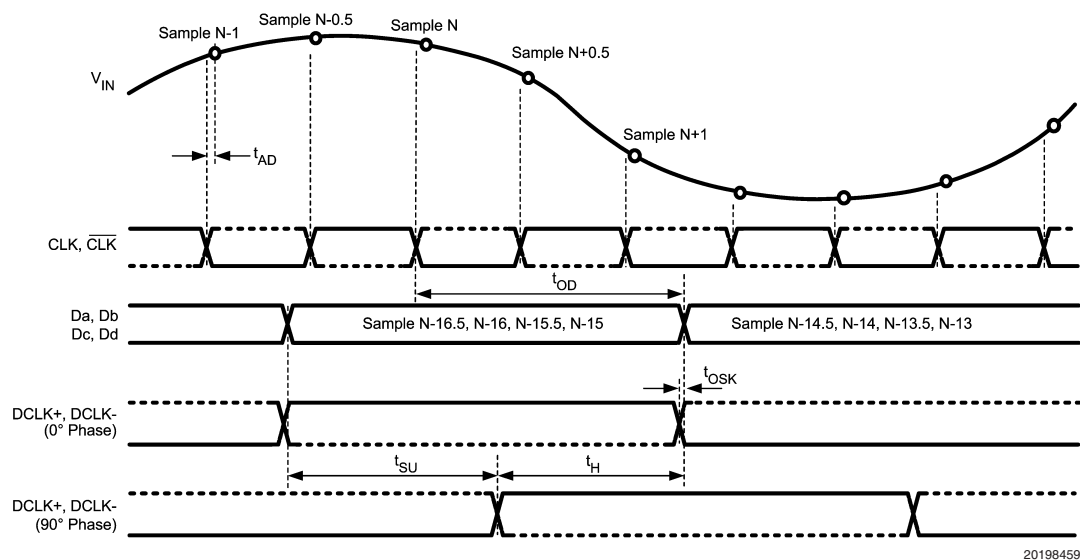
FIGURE 4. ADC082500 Timing — DDR Clocking
