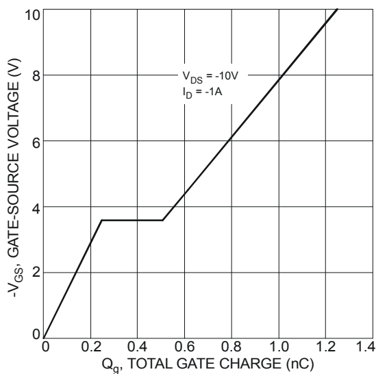
Figure 11 Gate-Charge Characteristics
