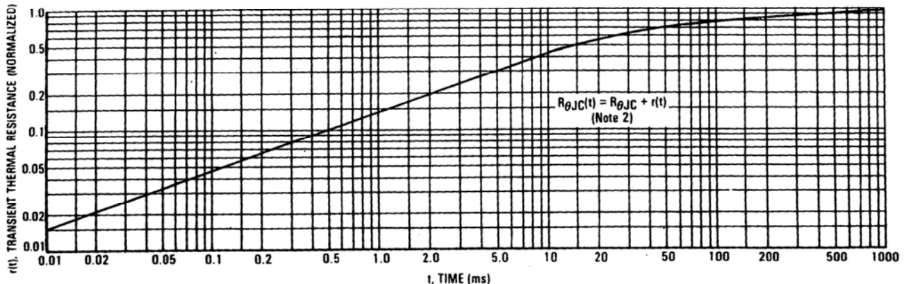
FIGURE 8 — THERMAL RESPONSE
