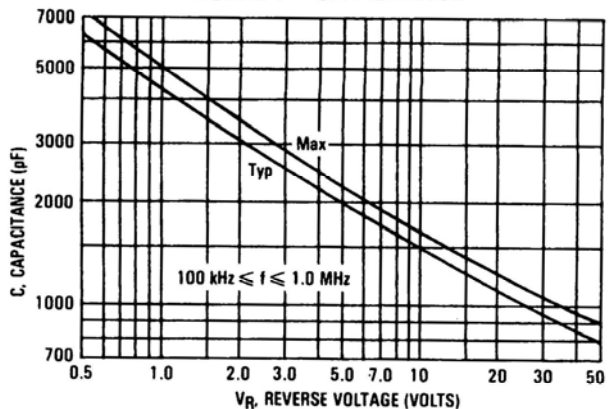
FIGURE 4 — CAPACITANCE
