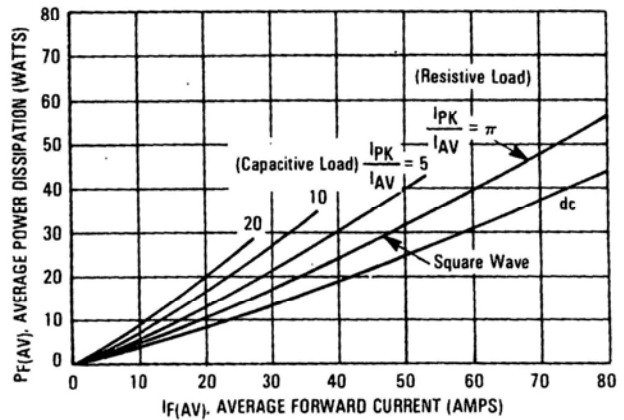
FIGURE 6 — POWER DISSIPATION
