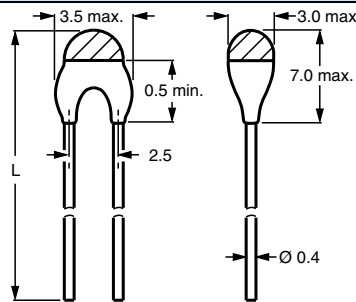
PTCSL20T..., L = 20 ± 2 PTCSL40T..., L = 40 min.
