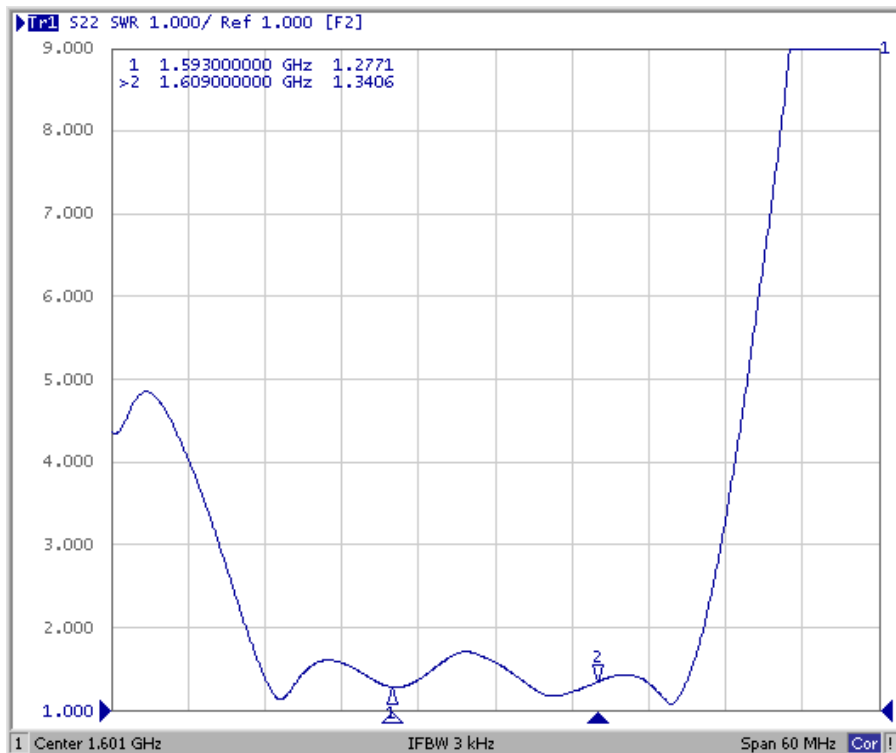
S22 VSWR
