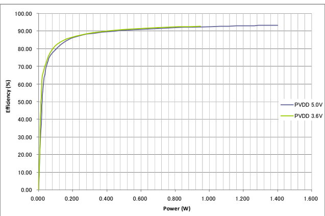
Figure 4. Efficiency into 8Ω + 33μH load
