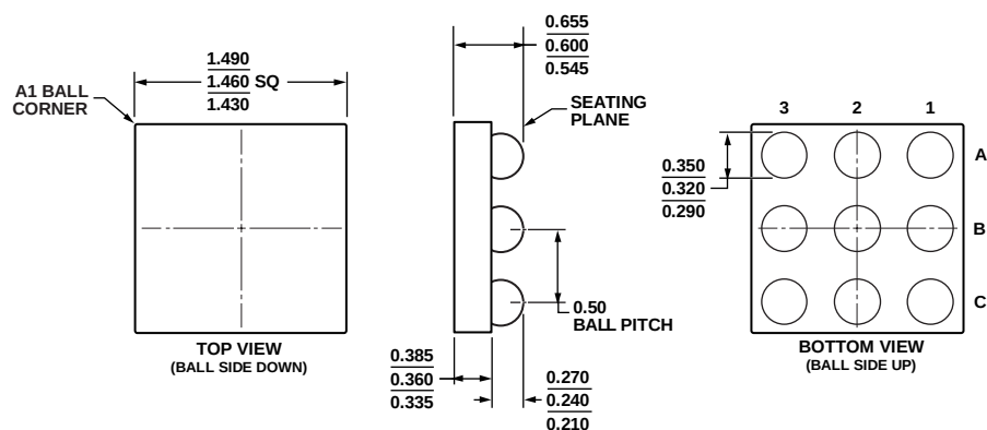
Figure 8. 9-Ball Wafer Level Chip Scale Package [WLCSP] (CB-9-2)
