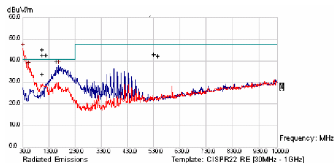
Figure 6. EMI Emissions from SSM2375, 50cm Cable, 5V V_{DD} , EDGE = V_{DD}
