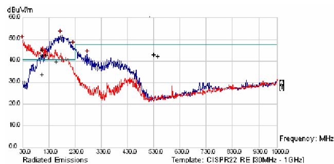
Figure 5. EMI Emissions from SSM2375, 50 cm Cable, 5V V_{DD} , EDGE = GND
