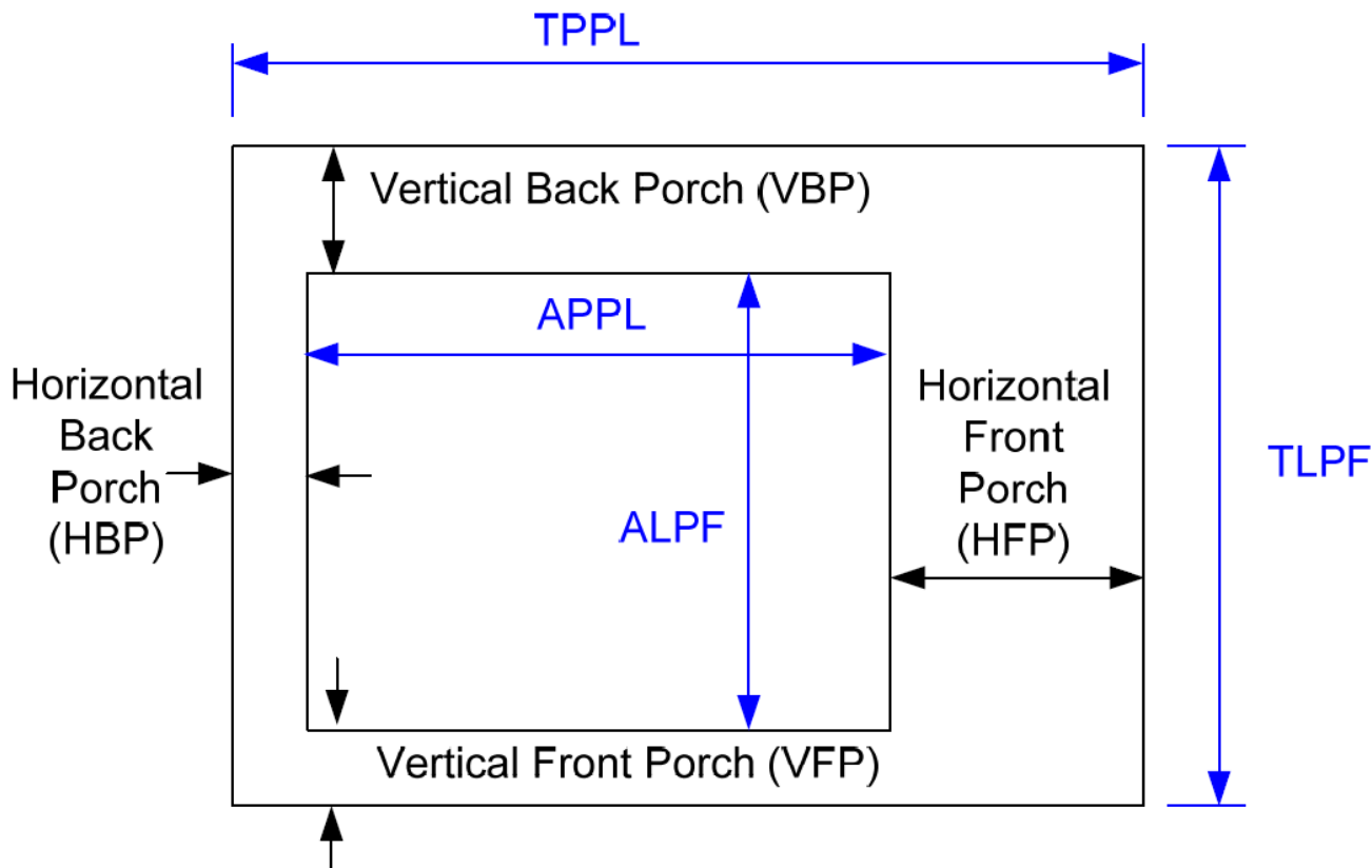
Figure 7. Horizontal and Vertical Blanking Diagram
